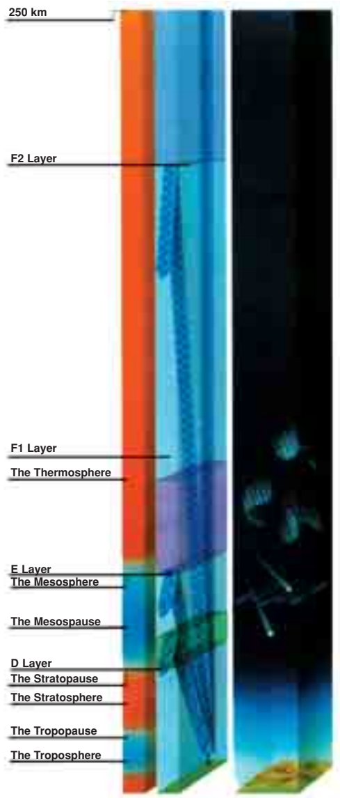
The layers of the atmosphere
